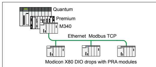
Modicon X80 DIO drops in a Quantum/Premium/M340 I/O architecture using Ethernet Modbus TCP
