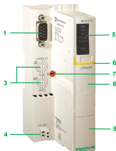
STBNC02212 CANOpen bus interface module
