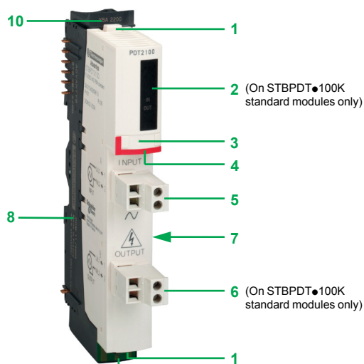
STB power distribution modules
