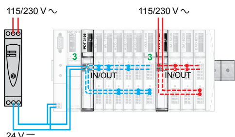
Configuration with basic PDM and one 24 V power supply
