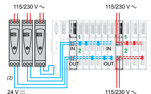
Configuration with standard PDM and three separate 24 V --- power supplies
